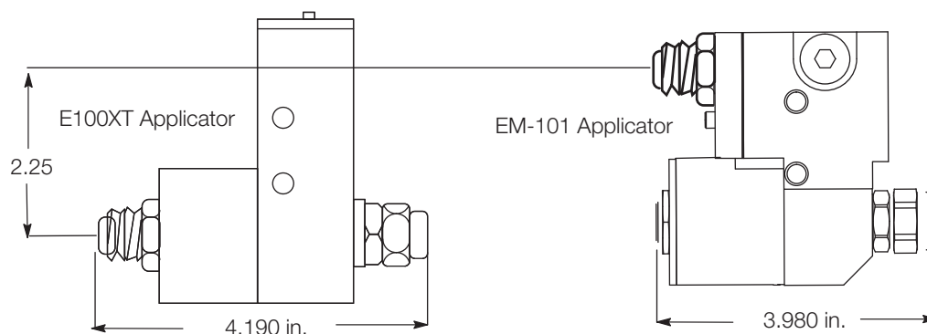
E-100XT to EM-101 Conversion Chart
