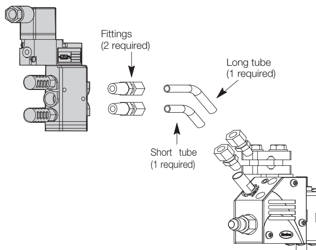
Air-Open/Air-Close (AO/AC) Configuration
