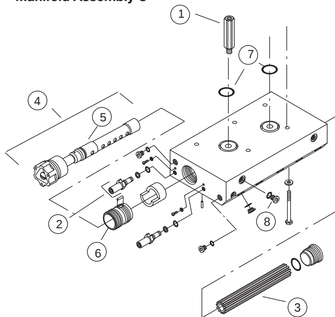
Manifold Assembly C
