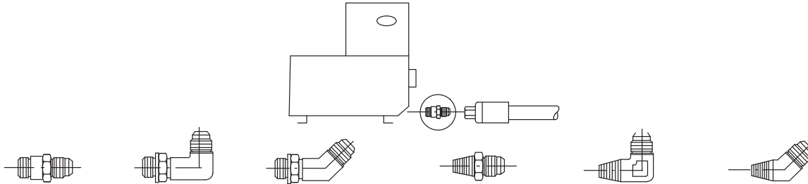
O-Ring Fitting (2000, 2300, 3000, 6000)
